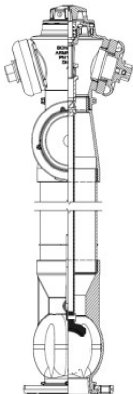
Hydrant otwarty
