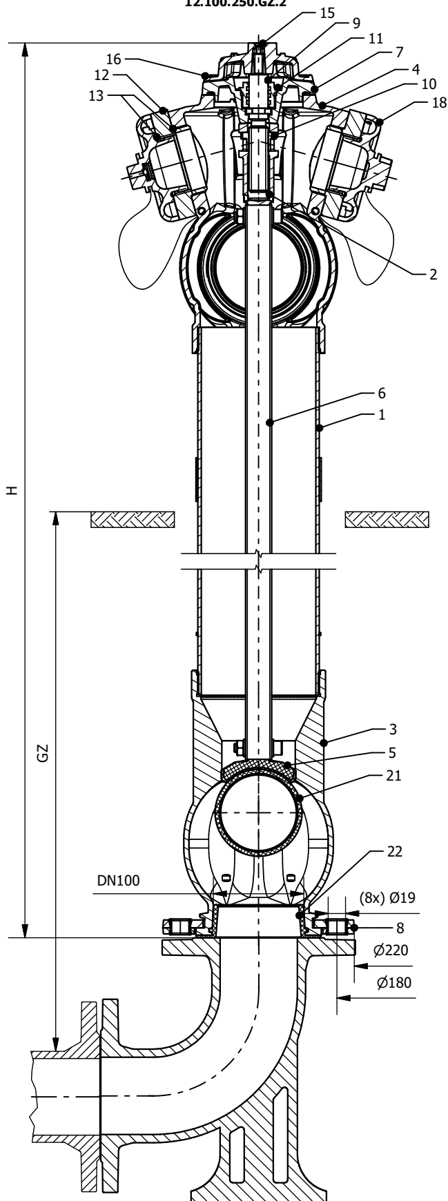
HN3-PW DN100 PN10/16 GJS 12.100.250.GZ.2
