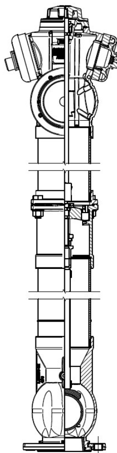
Hydrant otwarty
